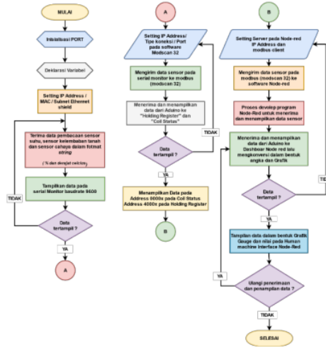
Gambar 10. Flowchart transfer data
