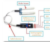
Gambar 3. Sensor kelembaban tanah YL-69
