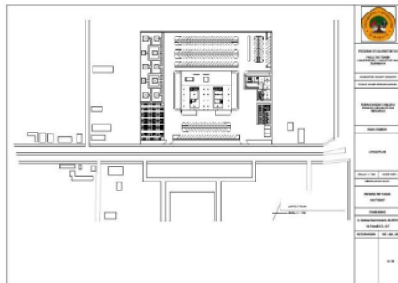
Gambar 14. Layout Plan
