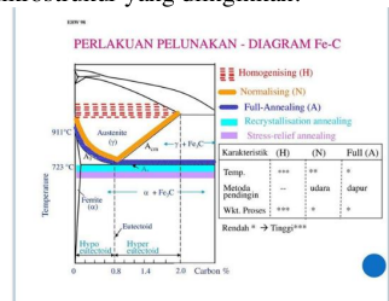
Gambar 2. 7 Diagram Annealing
