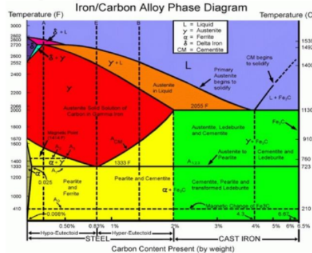
Gambar 2. 6 Diagram Fe3C
