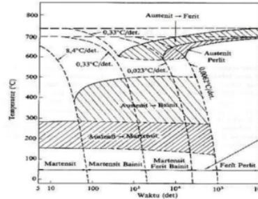
Gambar 2. 2 Diagram CCT
