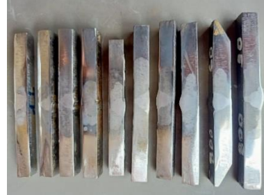
Gambar 4. 4 Proses etsa
