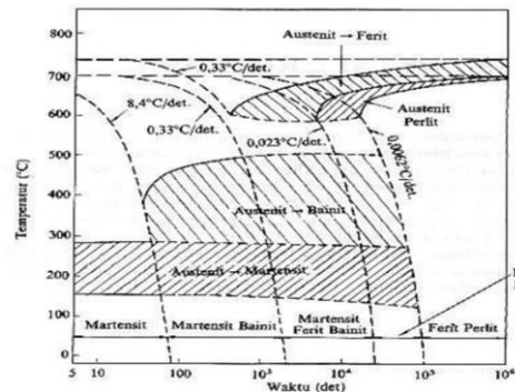
Gambar 2. 2 Diagram CCT
