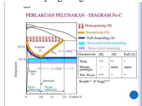
Gambar 2. 7 Diagram Annealing
