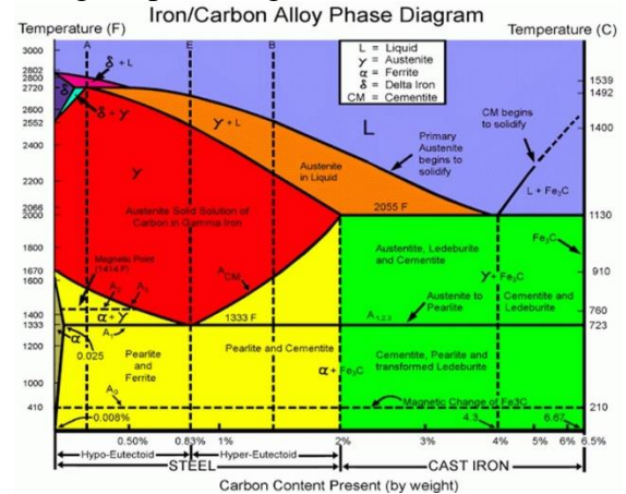
Gambar 2. 6 Diagram Fe3C
