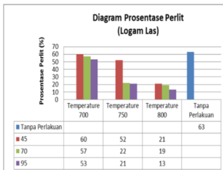
Gambar 4.10 Diagram Persentase Perlit
