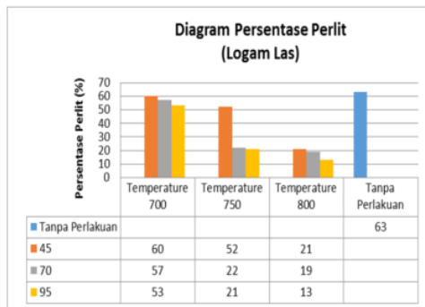
Gambar 4.6 Diagram Persentase Perlit
