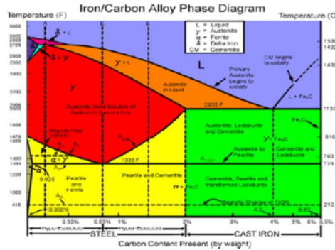
Gambar 2.5 Diagram Fe3C
