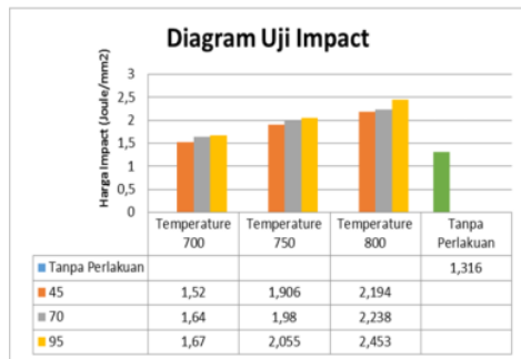
Gambar 4.7 Diagram Uji Impact
