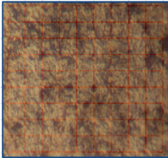
Gambar 4.5 Perhitungan Persentase Fasa
