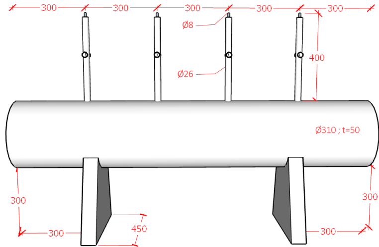
Tampak Samping
