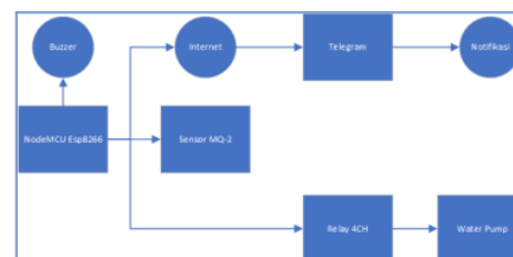
Gambar 2. Diagram Blok
