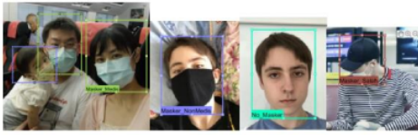
Gambar 7. Image Labelling
