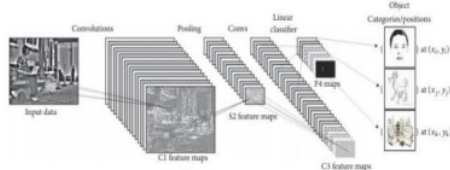
Gambar 3. Arsitektur Convolutional Neural Networks [15].
