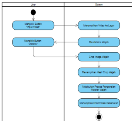
Gambar 5. Activity Diagram Sistem Deteksi Masker
