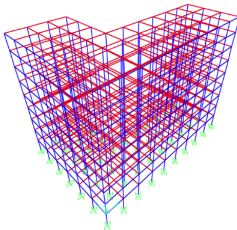
Gambar 2. 6 Gedung model takberaturan "L"
