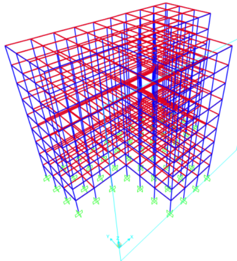
Gambar 2. 5 Gedung model takberaturan "T"
