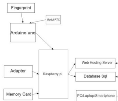
Gambar 2.1. Blok Diagram
