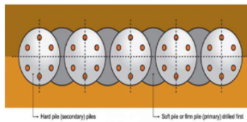
Gambar 4.2 Secant Pile (Sumber : Hardiyatmo, 2010)
