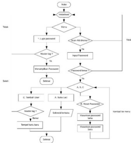
Gambar 7. Flowchart
