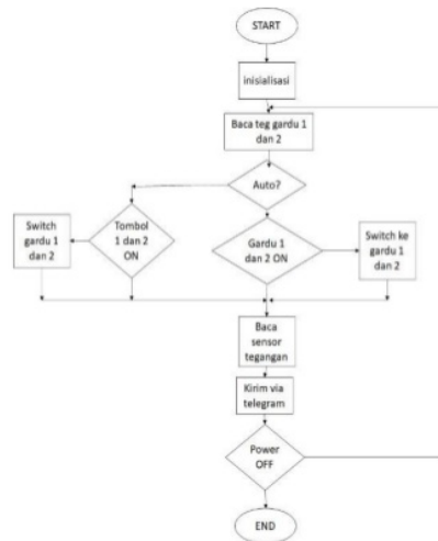
Gambar 5. Flowchart
