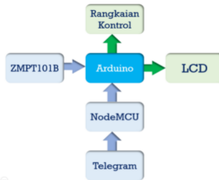
Gambar 8. Blok Diagram
