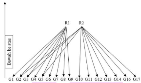
Gambar 2.1 Forward Chaining
