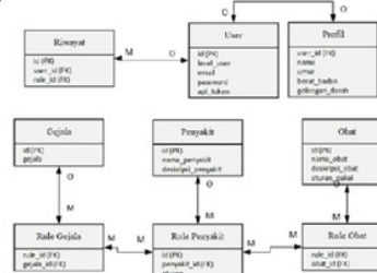
Gambar 2.14 ERD
