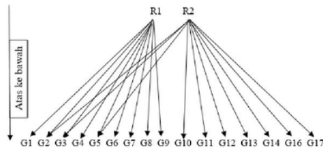
Gambar 2.2 Backward Chaining
