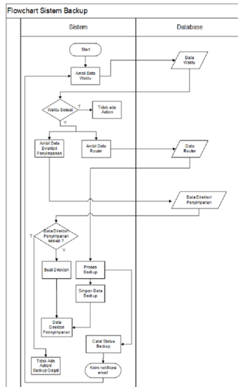
Gambar 7. Flowchart Sistem Backup
