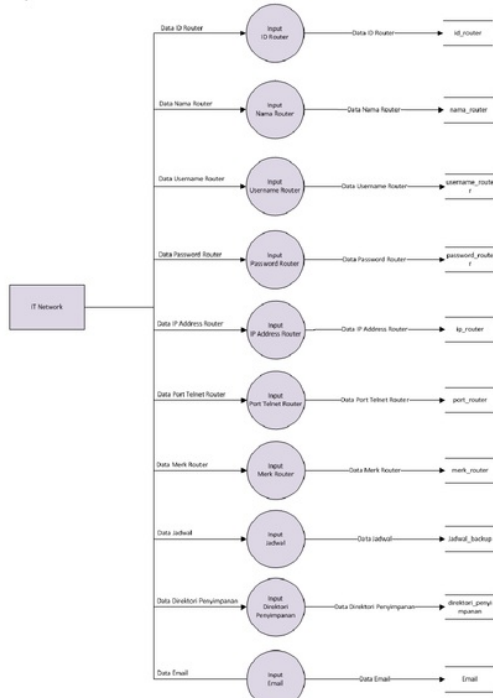
Gambar 11. Data Flow Diagram
