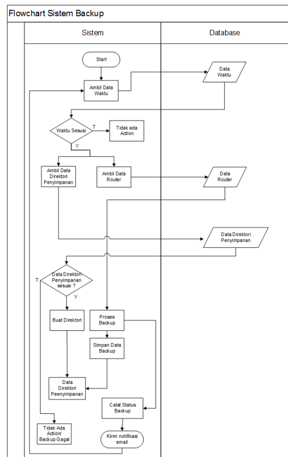
Gambar 7. Flowchart Sistem Backup
