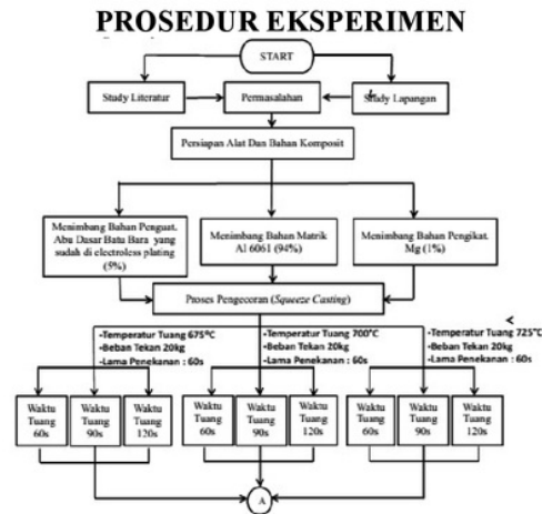
Gambar 7. Diagram Alir Prosedur Penelitian
