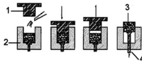
Gambar 1. Mekanisme Squeeze Casting
