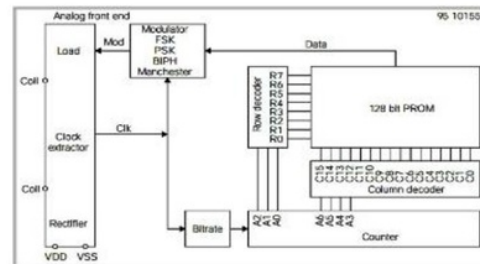
Gambar 3. Diagram Blok Passive Tag RFID (Finkenzeller 2003)
