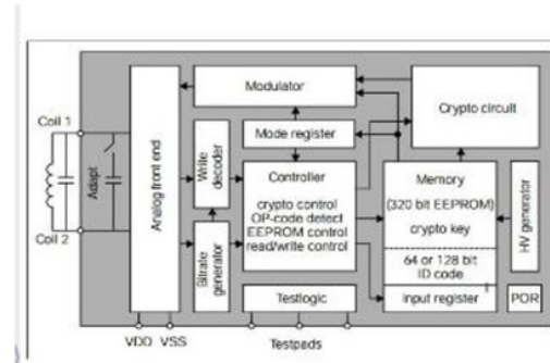
Gambar 2. Diagram Blok Active Tag RFID (Finkenzeller 2003)
