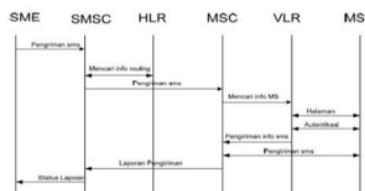
Gambar 6. Diagram Proses Pengiriman SMS
