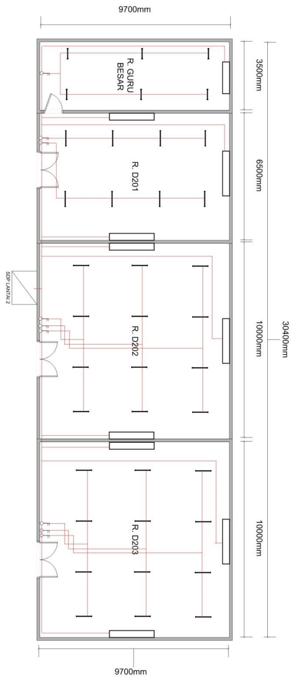
Gambar 2 Denah lantai 2
