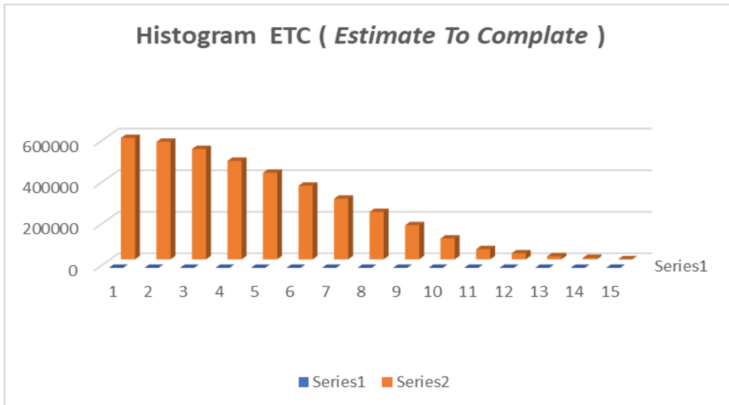
Gambar 4.4 Histogram ETC
