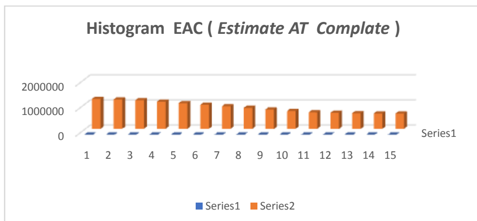
Gambar 4.5 Histogram EAC
