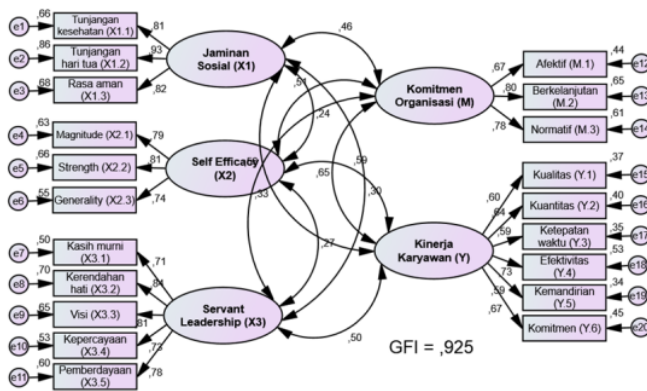
Gambar 2 Hasil CFA (Confirmatory Factor Analysis)
