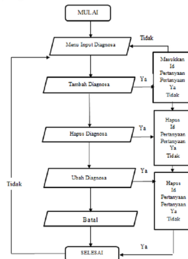
Gambar 1. Flowchart.
