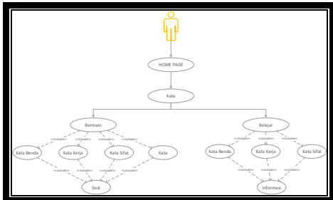
Gambar 2.1 Use Case Diagram
