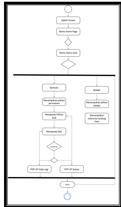
Gambar 2.2 Activity Diagram
