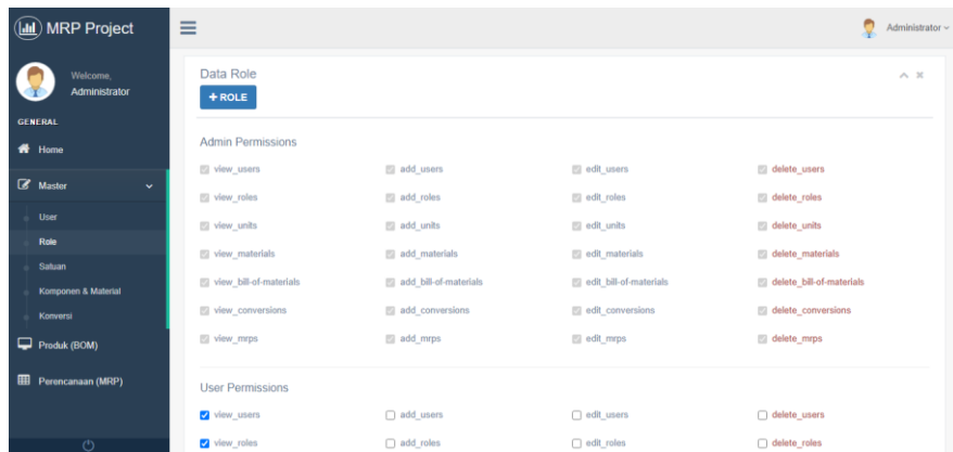
Tampilan Menu Master Role
