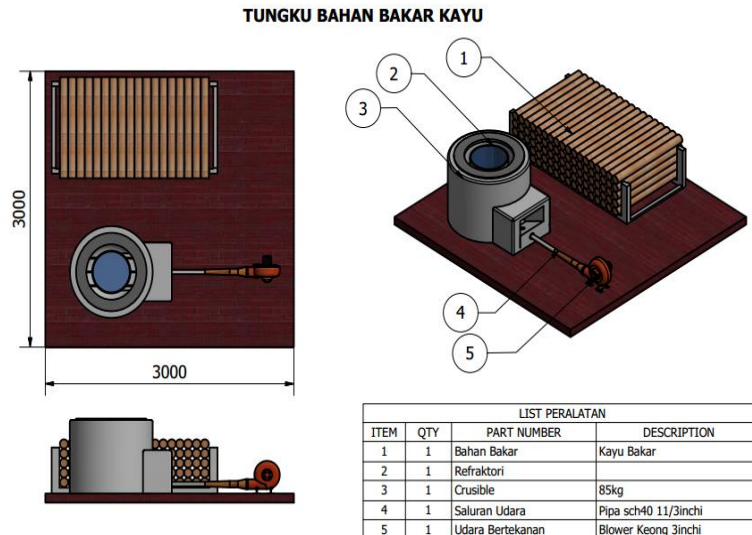
Gambar 3. Design Tungku Bahan bakar Kayu
