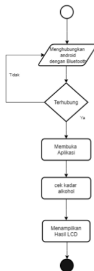
Gambar 3.1. Flowchart
