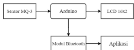
Gambar 2.1. Blok Diagram
