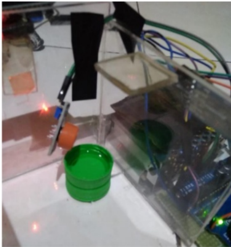
Gambar 3.3. Uji Coba Sensor MQ-3
