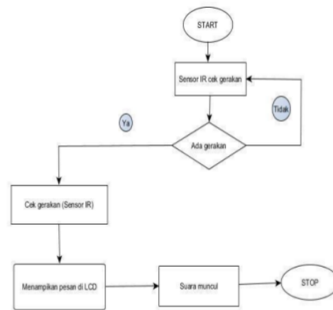
Gambar 2. Flowchart
