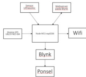
Gambar 1 Blok Diagram
