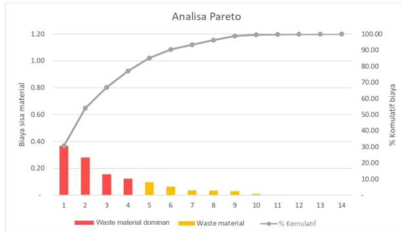
Gambar 3.1 Diagram Pareto
