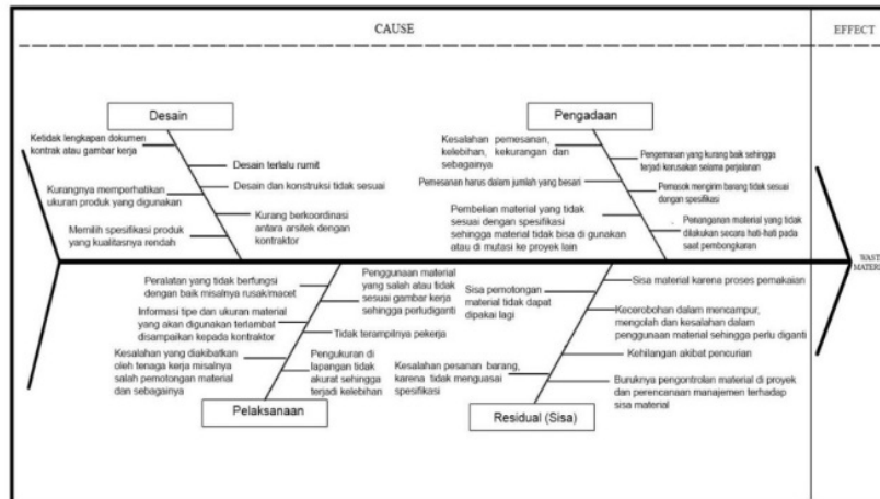
Gambar 3.2 Diagram Fishbone
