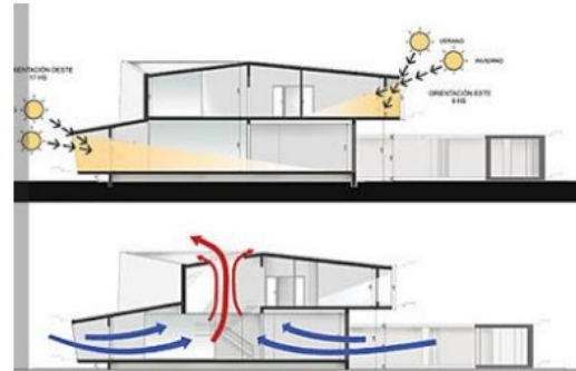
Gambar: Penerapan Cross Ventilation
