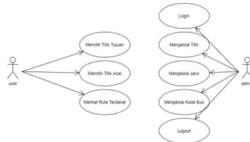
Gambar 3.3.1 Use Case Diagram
