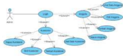
Gambar 3. Use Case Diagram Admin
