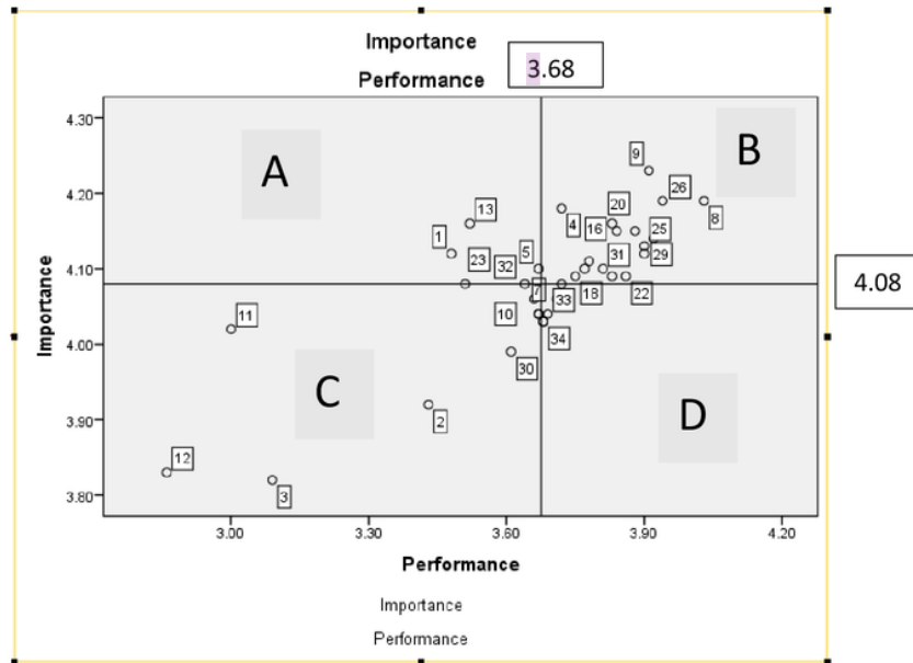
Gambar 3.2 Diagram Kartesius
