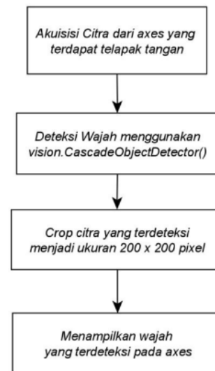
Gambar 4. Blok diagram metode viola jones
