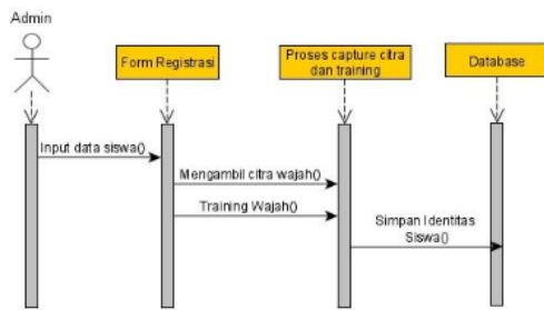
Gambar 13. Sequence Diagram Registrasi dan Training Wajah
