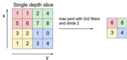
Gambar 8. Proses Max Pooling [12]
