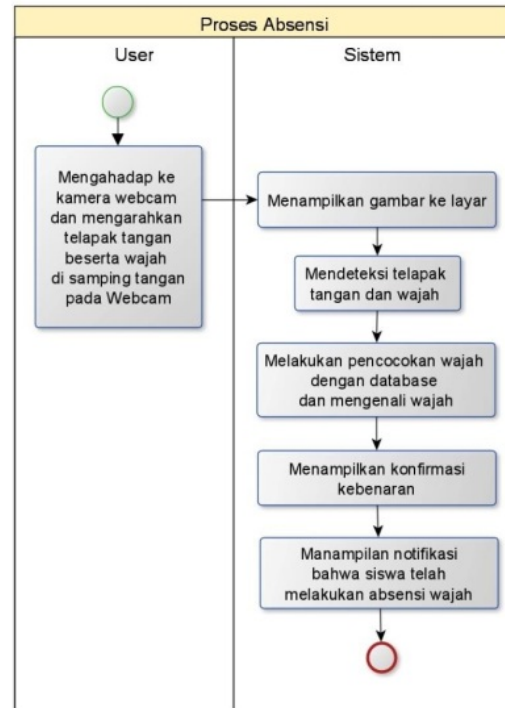
Gambar 12. Activity Diagram Proses Absensi
