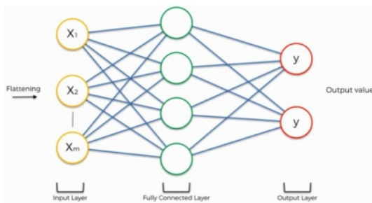
Gambar 9. Lapisan fully connected layer [12]
