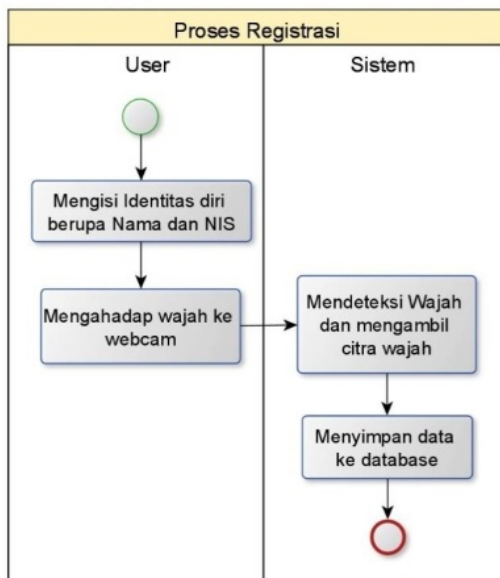
Gambar 11. Activity Diagram Proses Registrasi
