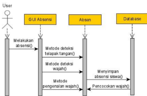
Gambar 14. Sequence Diagram
