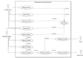
Gambar 3 Diagram Use Case
