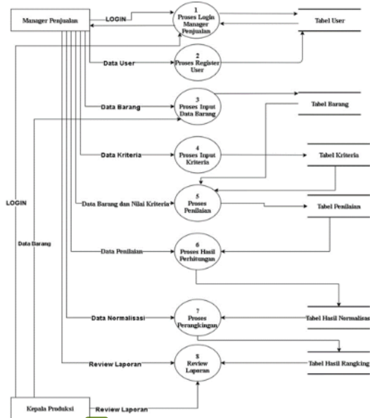
Gambar 2 Data Flow Diagram (DFD) Level 1
