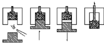
Gambar 1. Mekanisme Squeeze Casting
