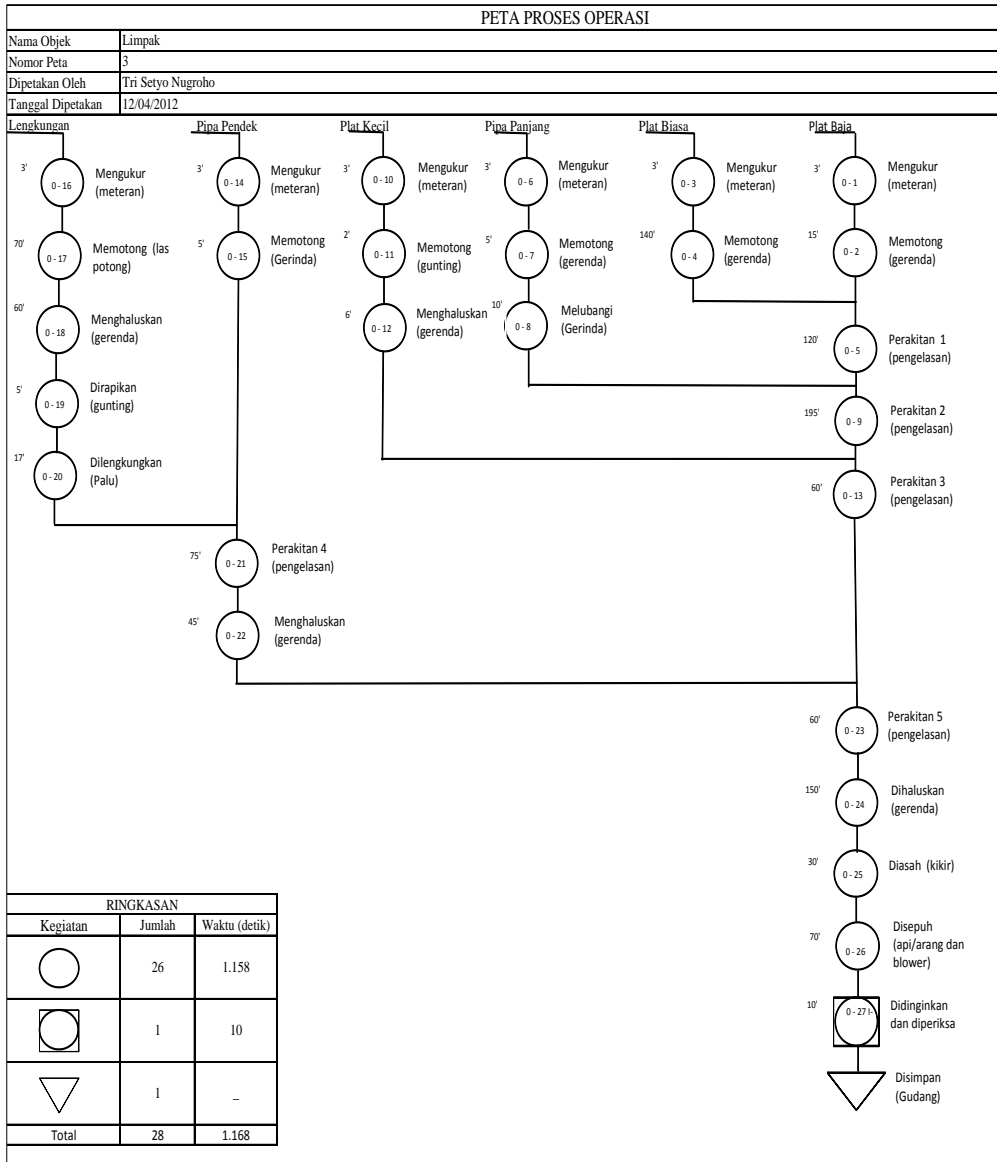
Gambar 9 peta proses operasi limpak
