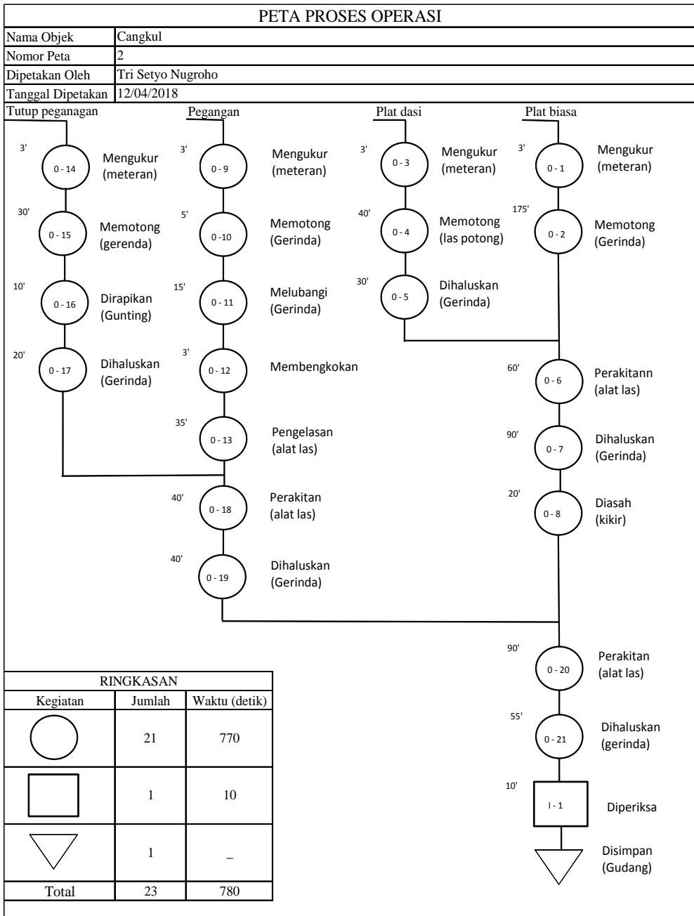
Gambar 8 peta proses operasi cangkul
