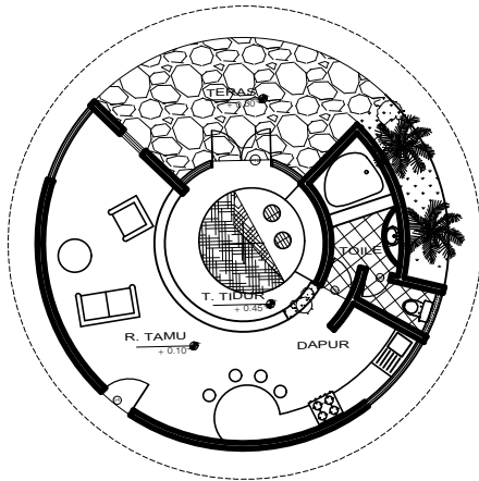
DENAH COTTAGE
