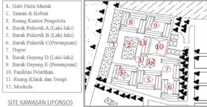
Gambar 3.2 Lay out eksisting UPTD.LIPONSOS
