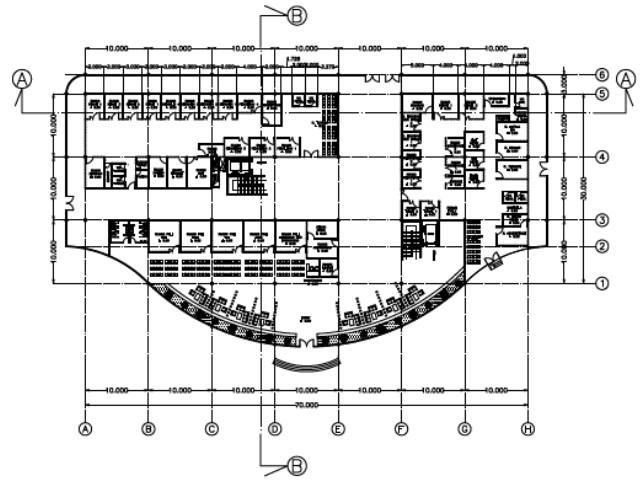
DENAH L1 MASSA 1 Skala 1:200
