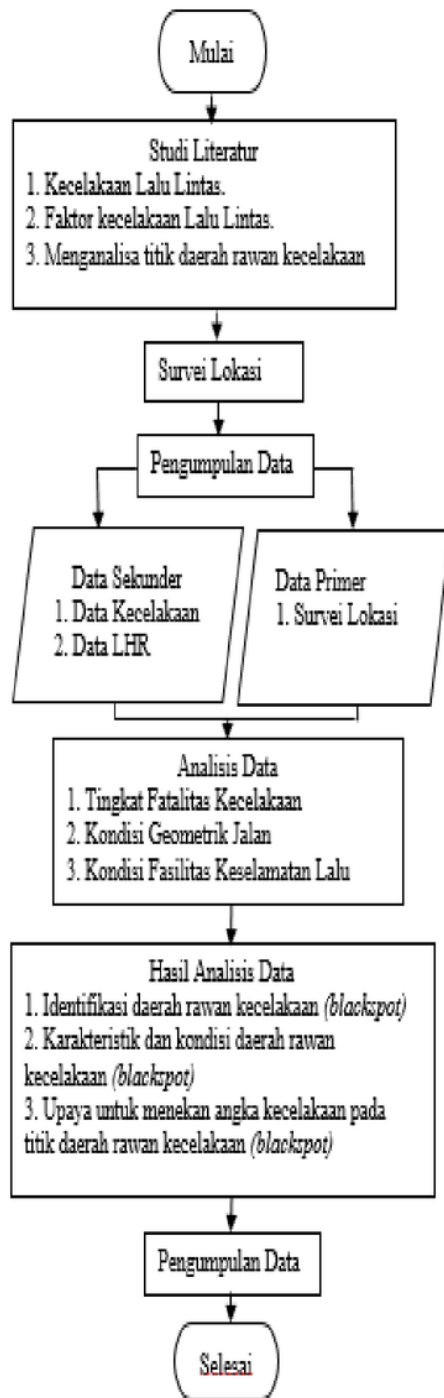
Gambar 1. Flowchart
