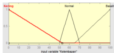
Gambar 2.2 Membership Variabel Kelembapan
