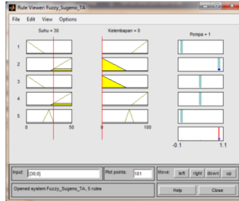
Gambar 4.1. Simulasi Fuzzy Matlab
