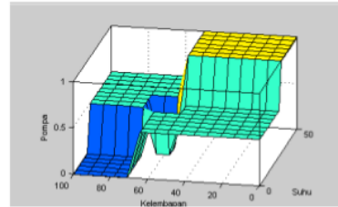
Gambar 2.3 Tampilan Surface FIS Matlab
