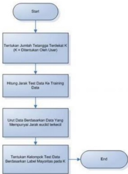
Gambar 6 Flowchart Metode K-NN
