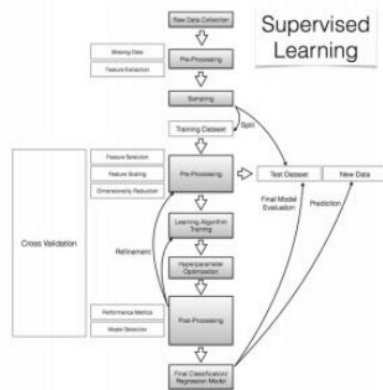
Gambar 4 Flowchart Supervised Learning
