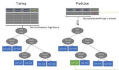
Gambar 7 Flowchart Metode Decision Tree
