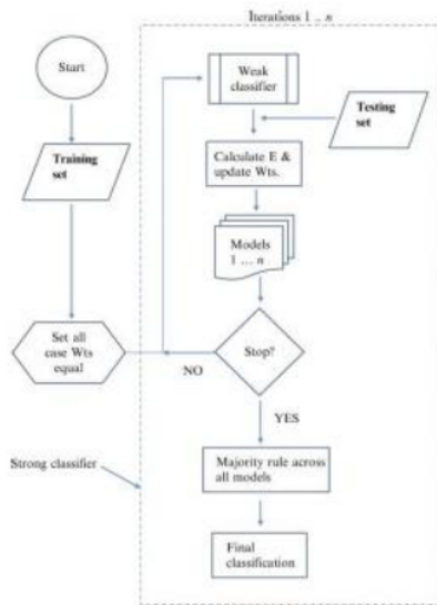
Gambar 10 Flowchart Metode Gradient Boosting
