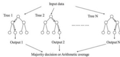
Gambar 8 Flowchart Metode Random Forest
