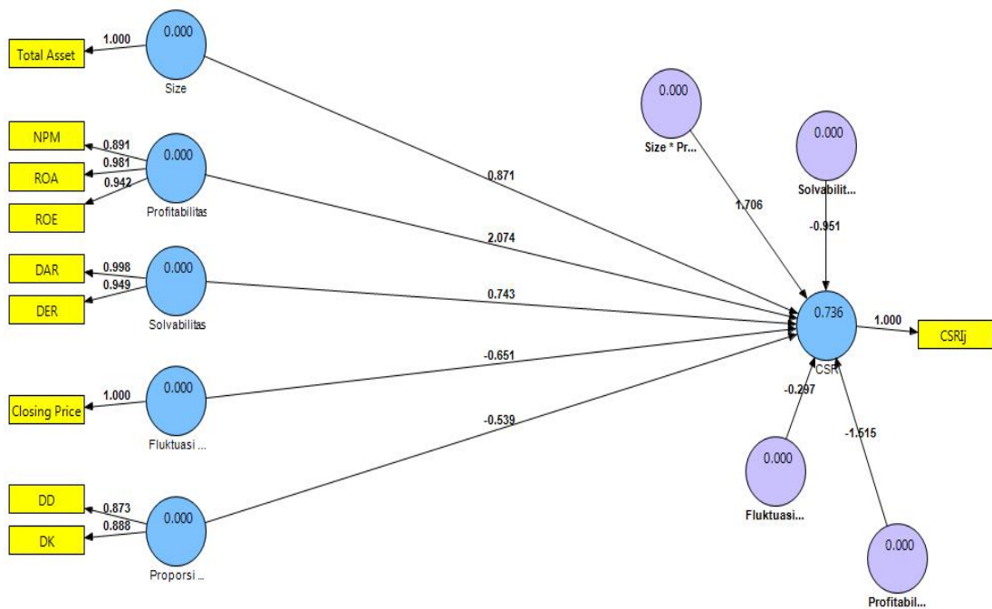
Gambar 5.2 Outer Loading re-estimasi
