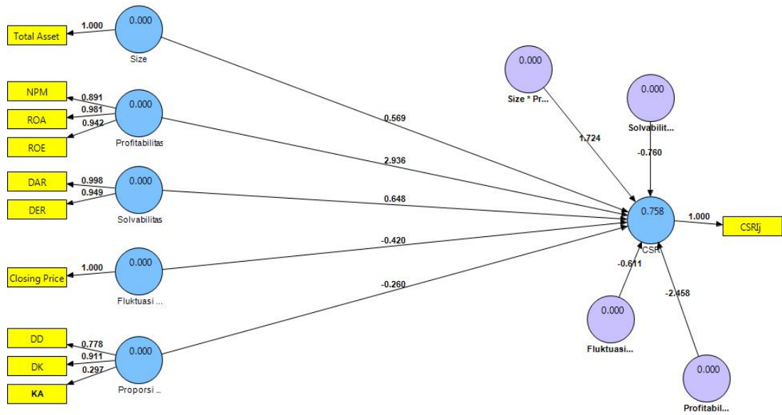
Gambar 5.1 Outer Loading
