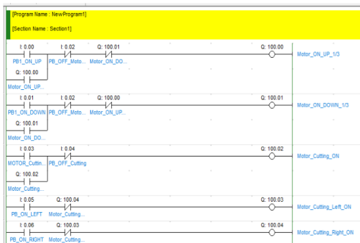
PROGRAM LEADDER PLC OMRON CP1L
