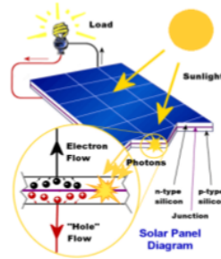
Gambar 2.1 Prinsip kerja panel surya
