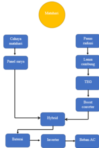
Gambar 3.2 Blok diagram sistem hybrid
