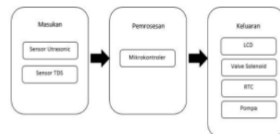
Gambar 3.1 blok diagram
