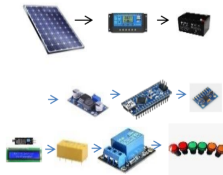
Gambar 2. Desain Hardware
