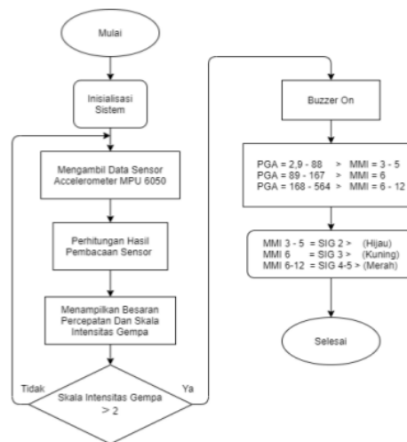
Gambar 3. Flowchart
