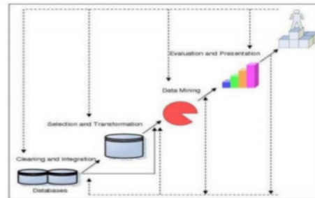
Gambar 2 Data Mining
