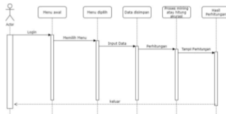
Gambar 12 Squence diagram user
