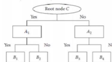
Gambar 3 Decision Tree
